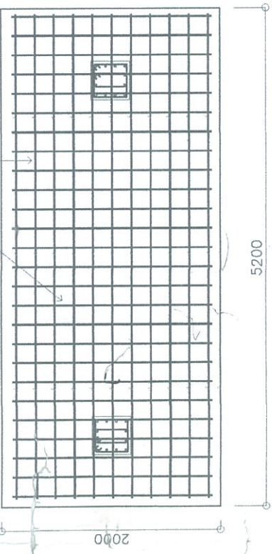
PEDESTAL ELEVATION
